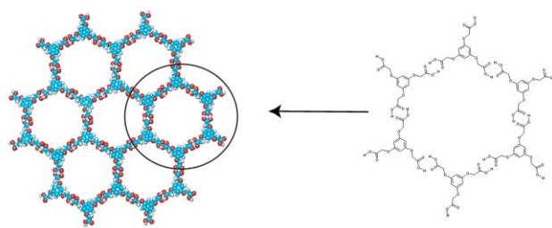
Fig. 2 Simulated molecular model representing the assembly structure of TCMB.
