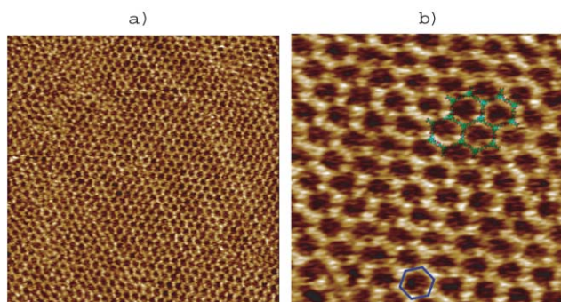
Fig. 1 (a) STM image ( 66 \times 66 \text{ nm}^2 ) of a self-assembled monolayer of TCMB on a HOPG surface. The imaging conditions are I = 877 \text{ pA} and V = 641 \text{ mV} . The z -axis is 0.5 \text{ nm} . (b) A higher resolution STM image ( 19 \times 19 \text{ nm}^2 ) of TCMB. The imaging conditions are I = 766 \text{ pA} and V = 341 \text{ mV} . The z -axis is 0.5 \text{ nm} .
